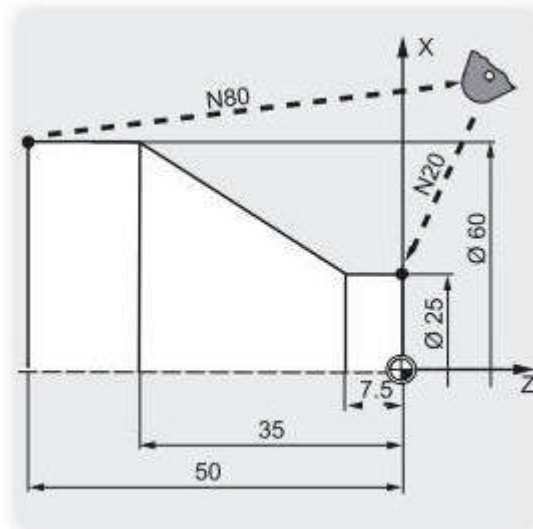
Lathe CNC Programming Example
